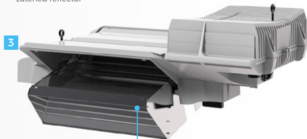
Unlatched reflector
